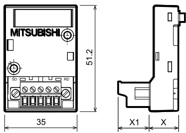
FX3G-485-BD
