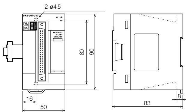
FX5-20PG-D
