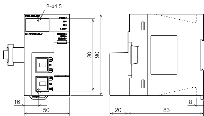
FX5-CCLIEF
