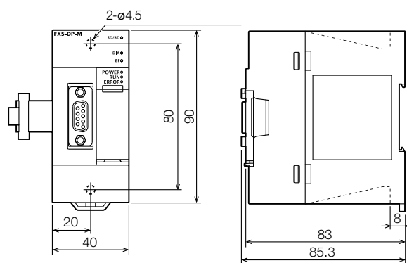
FX5-DP-M
