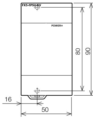
FX5-1PSU-5V
