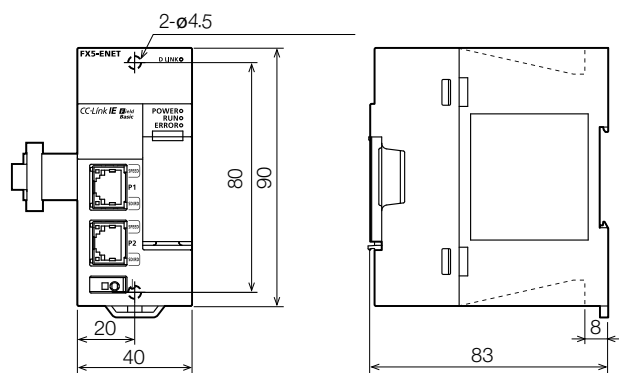
FX5-ENET,
