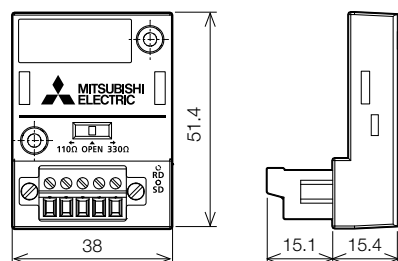
FX5-485-BD
