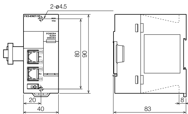
FX5-ENET/IP
