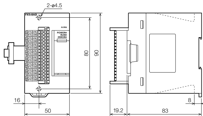
FX5-8AD
