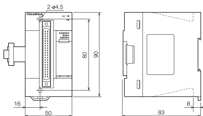
FX5-20PG-P
