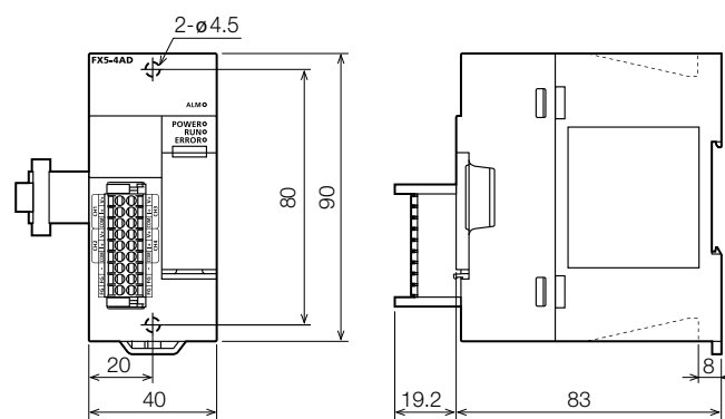
FX54AD, FX5-4DA
