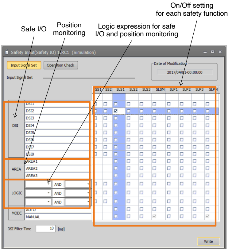
Safety logic editing screen
