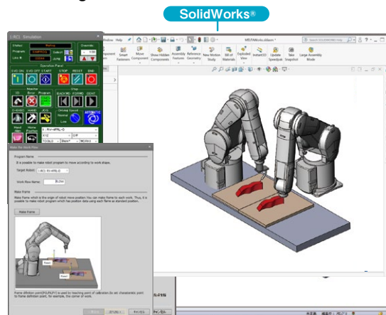
Calibration tool
